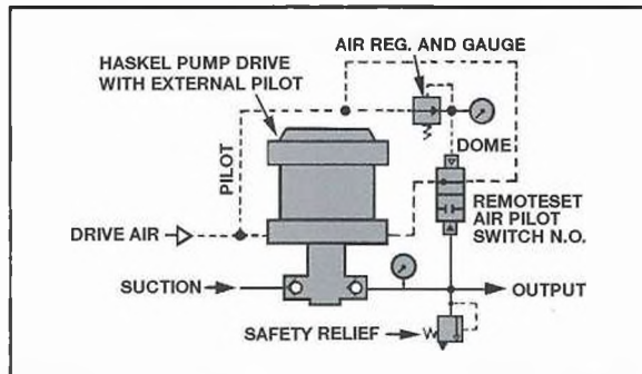
3. Maximum output pressure control remote, air adjusted
